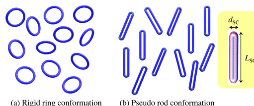
Figure 2. Schematic representation of the rigid ring polymer.
