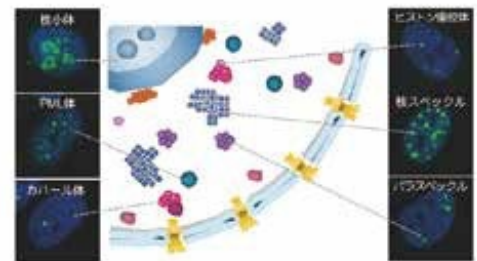
Figure 2: Schematic diagram of membraneless structures in mammalian cell nuclei
